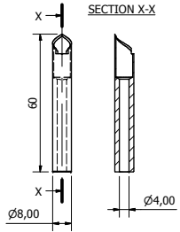
AP0860-1 Ø8.00 x 60mm LONG Ø4.00 THROUGH HOLE
