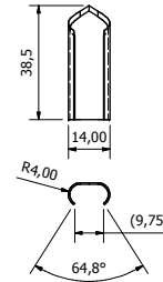
AP3914-8 14mm OVAL 38.5mm LONG
