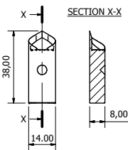
AP1408-4 14x8mm OVAL 38mm LONG
