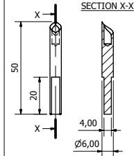
AP5006-1 Ø6.00mm x 50mm LONG WITH FLATS
