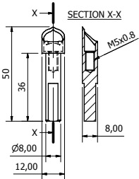
AP5012-2 12x8mm OVAL 50mm LONG, M5 HOLE
