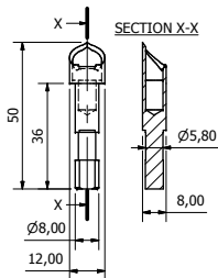
AP5012-5D 12x8mm OVAL 50mm LONG WITH GROOVE
