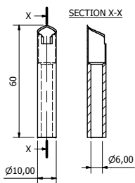
AP6010-1 Ø10mm x 60mm LONG Ø6mm THROUGH HOLE
