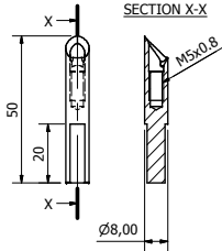
AP5008-1 Ø8mm x 50mm LONG WITH FLATS & M5 HOLE
