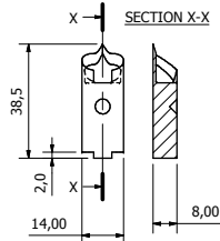
AP1408-2 OVAL 14.00x8.00mm x 38.50mm LONG
