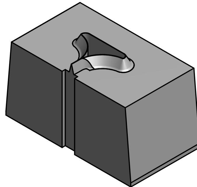
HS4022-2T HALF STAR R8,00 22x40mm, 23,70mm HIGH WITH 5° TAPERED SIDES TO SUIT 4mm CUTTING RULE
