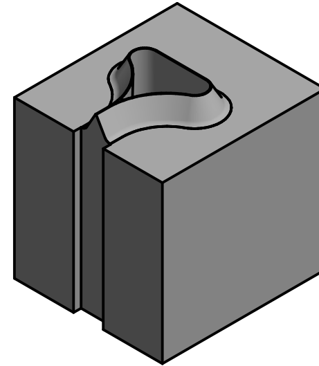
HS4004-R1.5 HALF STAR R8,00 22x20mm, 23,70mm HIGH TO SUIT 4mm CUTTING RULE
