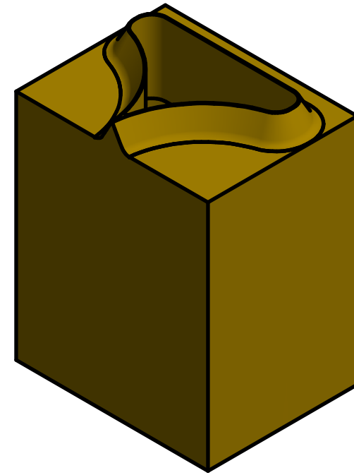
THS1005-2 HALF STAR R9,65 14x18mm, 23,80mm HIGH TiN COATED
